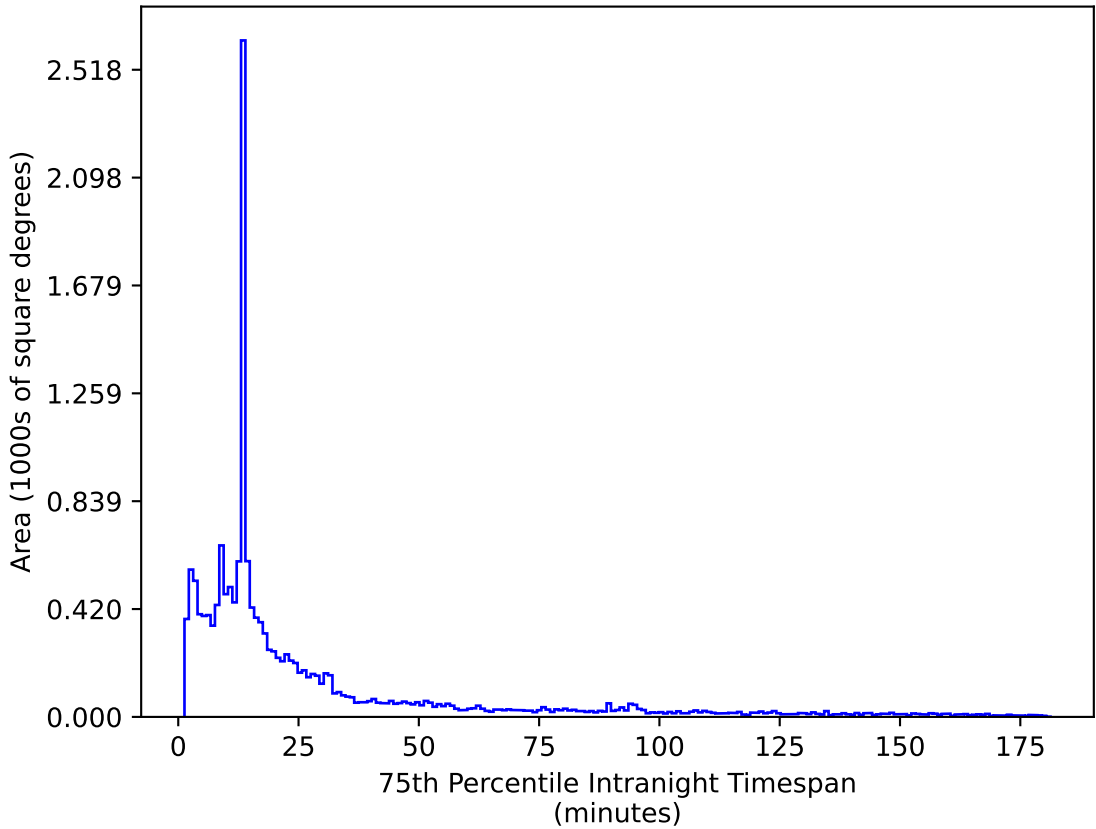
too_elab_r256_d3_griz_v3.4_10yrs WFD z band: 75th Percentile Intranight Timespan
