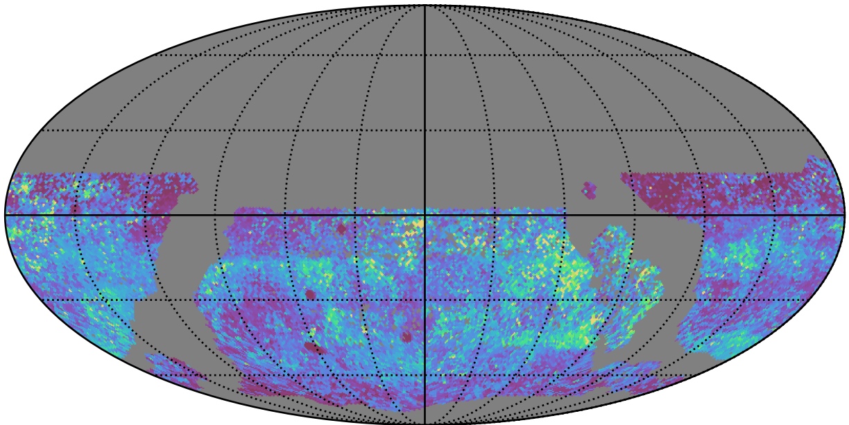
too_elab_r256_d3_griz_v3.4_10yrs WFD y band: 75th Percentile Intranight Timespan
