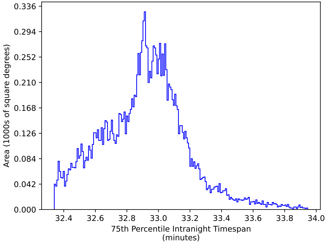
too_elab_r256_d3_griz_v3.4_10yrs WFD y band: 75th Percentile Intranight Timespan
