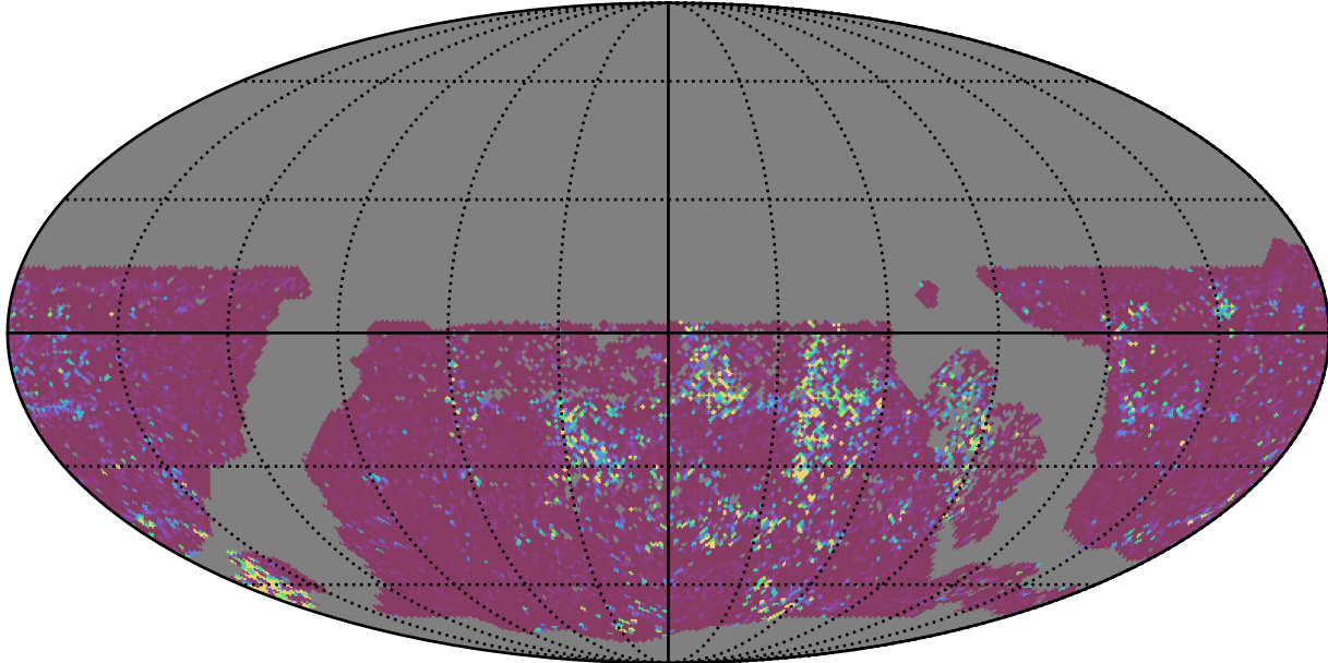
too_elab_r256_d3_griz_v3.4_10yrs WFD u band: 75th Percentile Intranight Timespan
