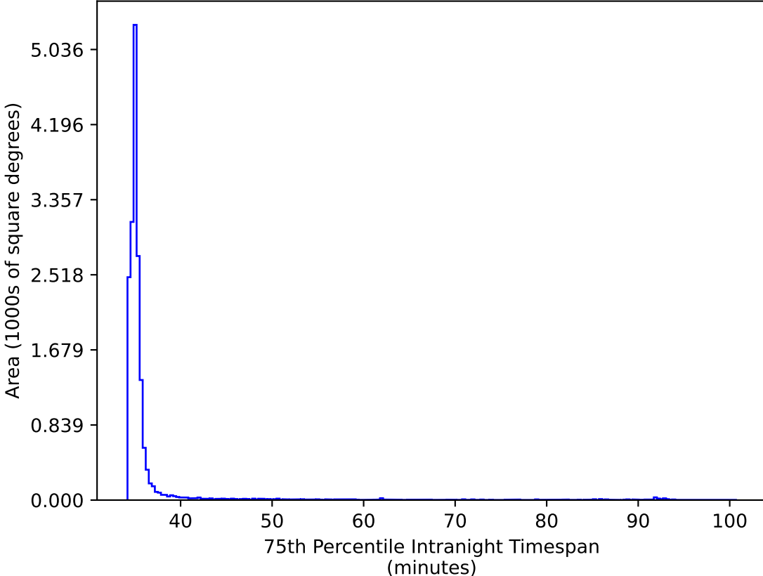
too_elab_r256_d3_griz_v3.4_10yrs WFD ri bands: 75th Percentile Intranight Timespan
