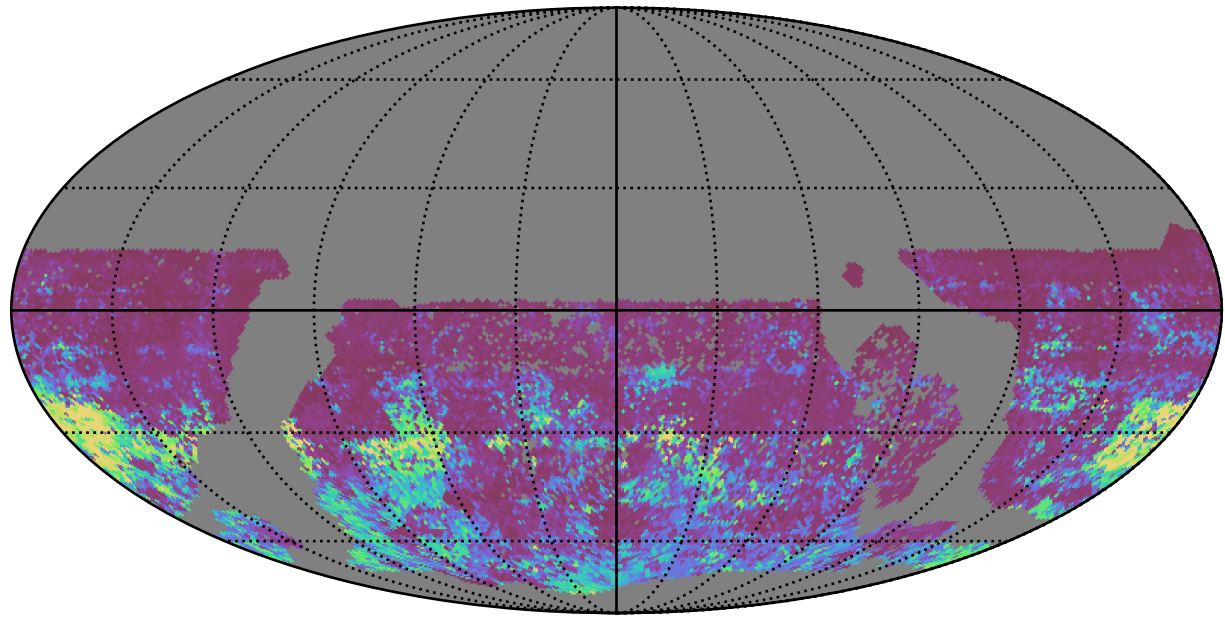
too_elab_r256_d3_griz_v3.4_10yrs WFD r band: 75th Percentile Intranight Timespan
