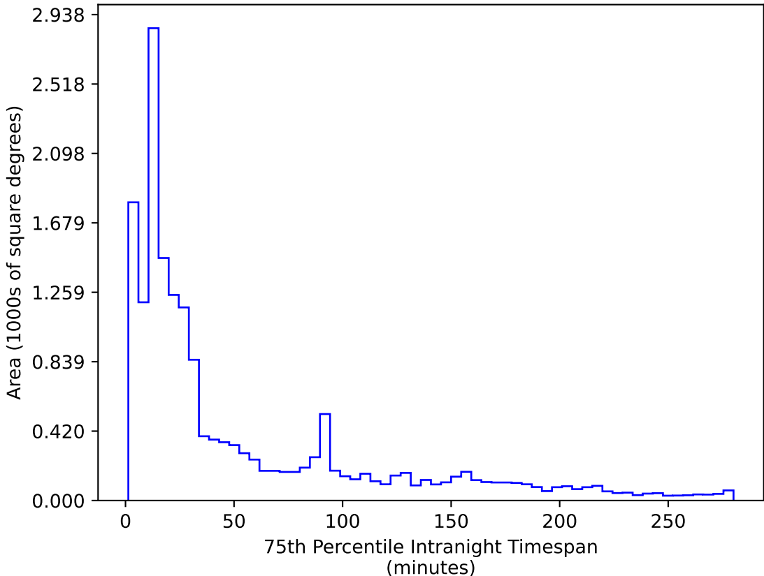
too_elab_r256_d3_griz_v3.4_10yrs WFD r band: 75th Percentile Intranight Timespan
