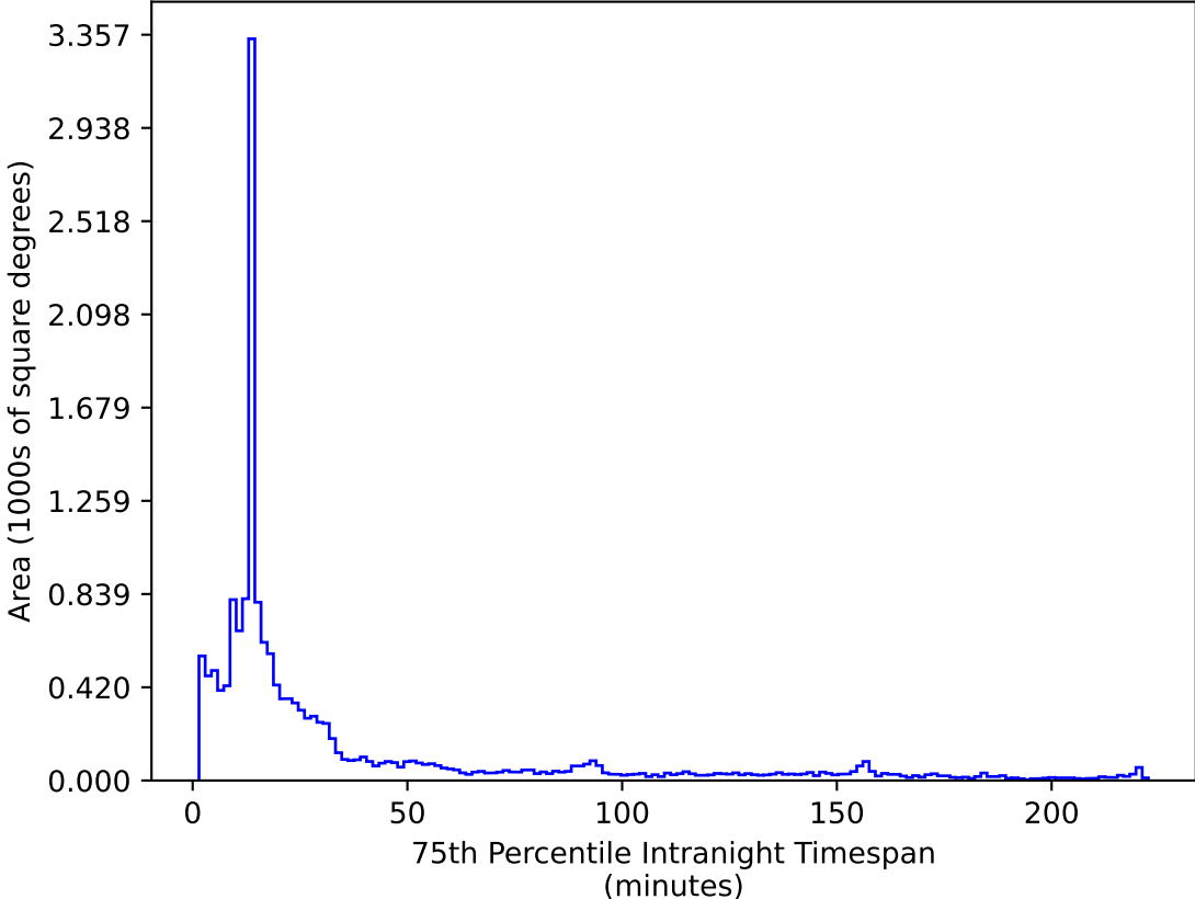
too_elab_r256_d3_griz_v3.4_10yrs WFD i band: 75th Percentile Intranight Timespan
