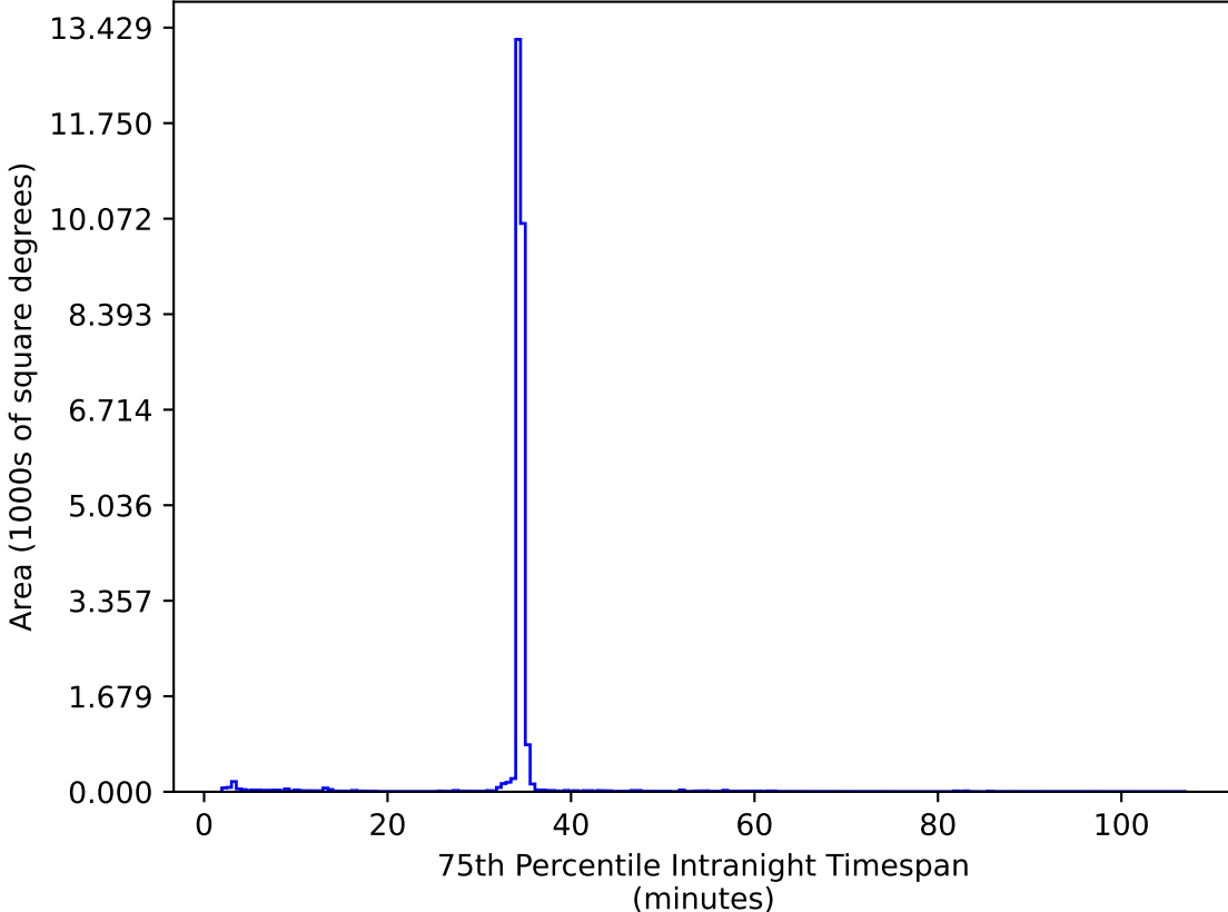
too_elab_r256_d3_griz_v3.4_10yrs All sky zy bands: 75th Percentile Intranight Timespan
