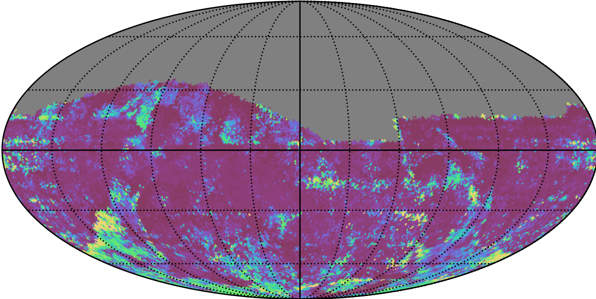
too_elab_r256_d3_griz_v3.4_10yrs All sky z band: 75th Percentile Intranight Timespan
