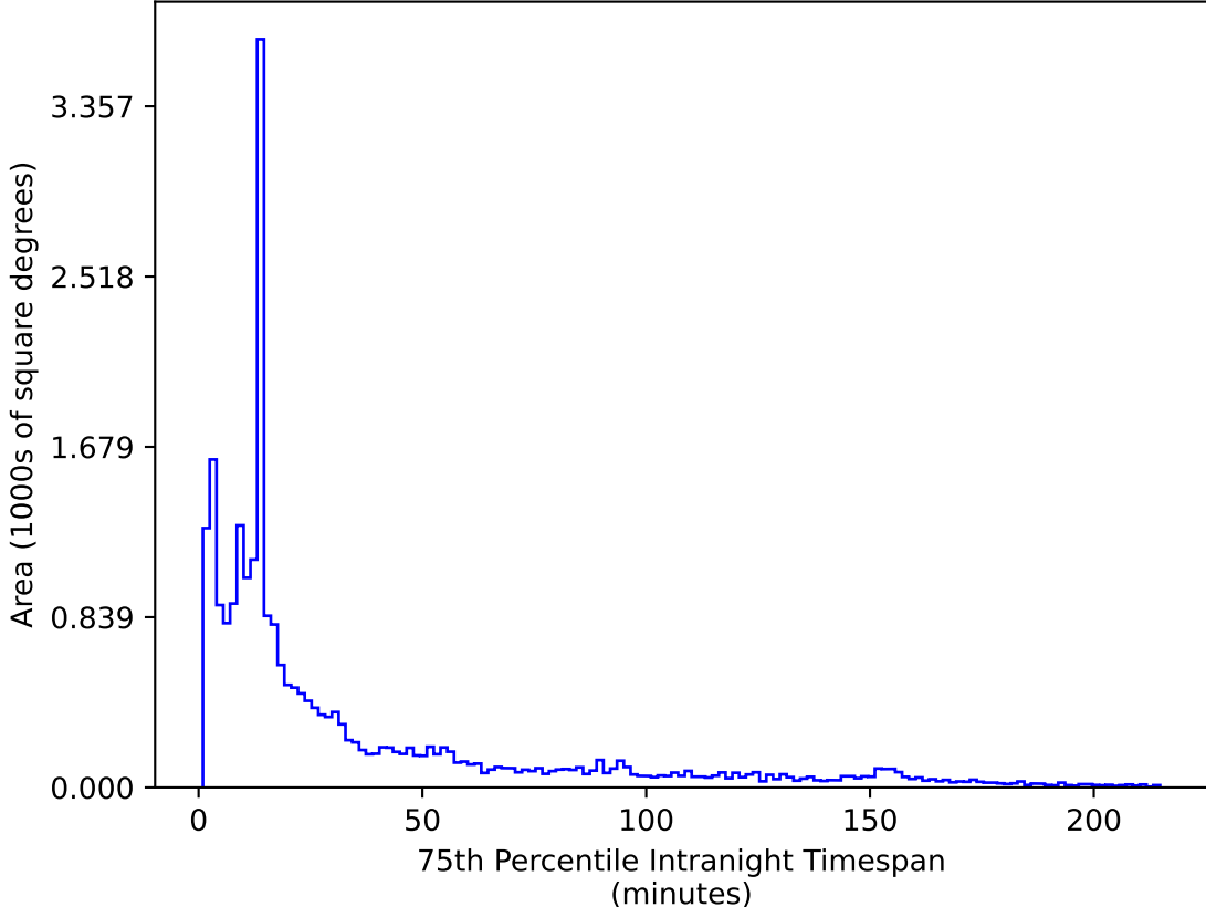
too_elab_r256_d3_griz_v3.4_10yrs All sky z band: 75th Percentile Intranight Timespan
