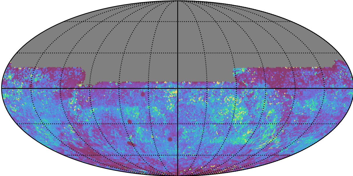
too_elab_r256_d3_griz_v3.4_10yrs All sky y band: 75th Percentile Intranight Timespan
