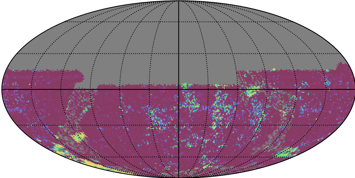
too_elab_r256_d3_griz_v3.4_10yrs All sky u band: 75th Percentile Intranight Timespan
