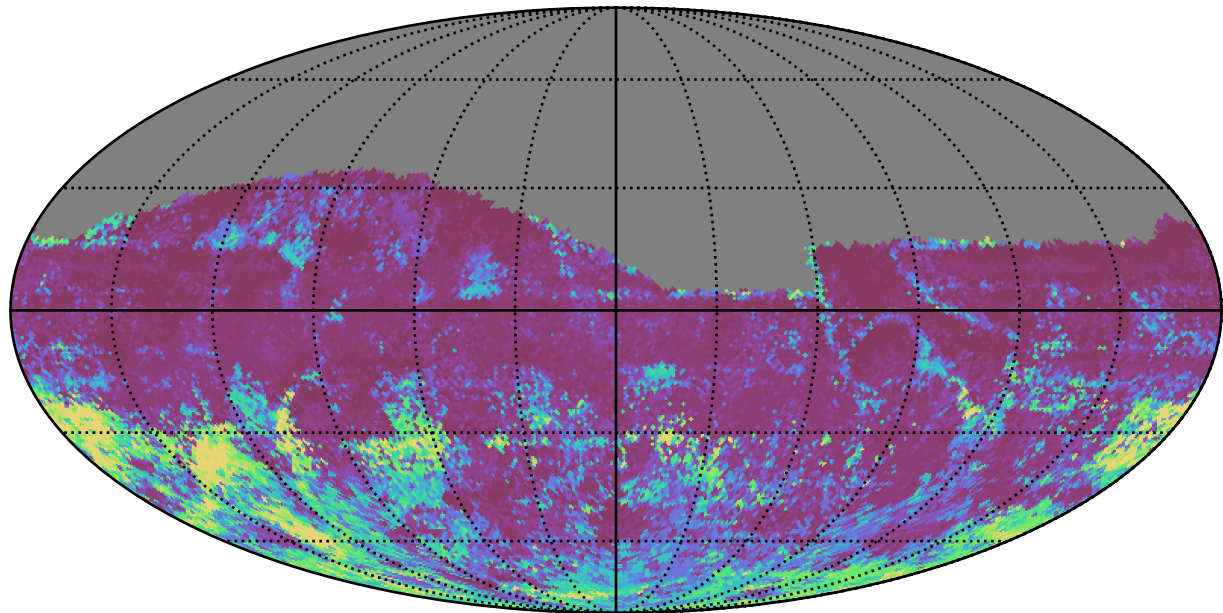
too_elab_r256_d3_griz_v3.4_10yrs All sky r band: 75th Percentile Intranight Timespan
