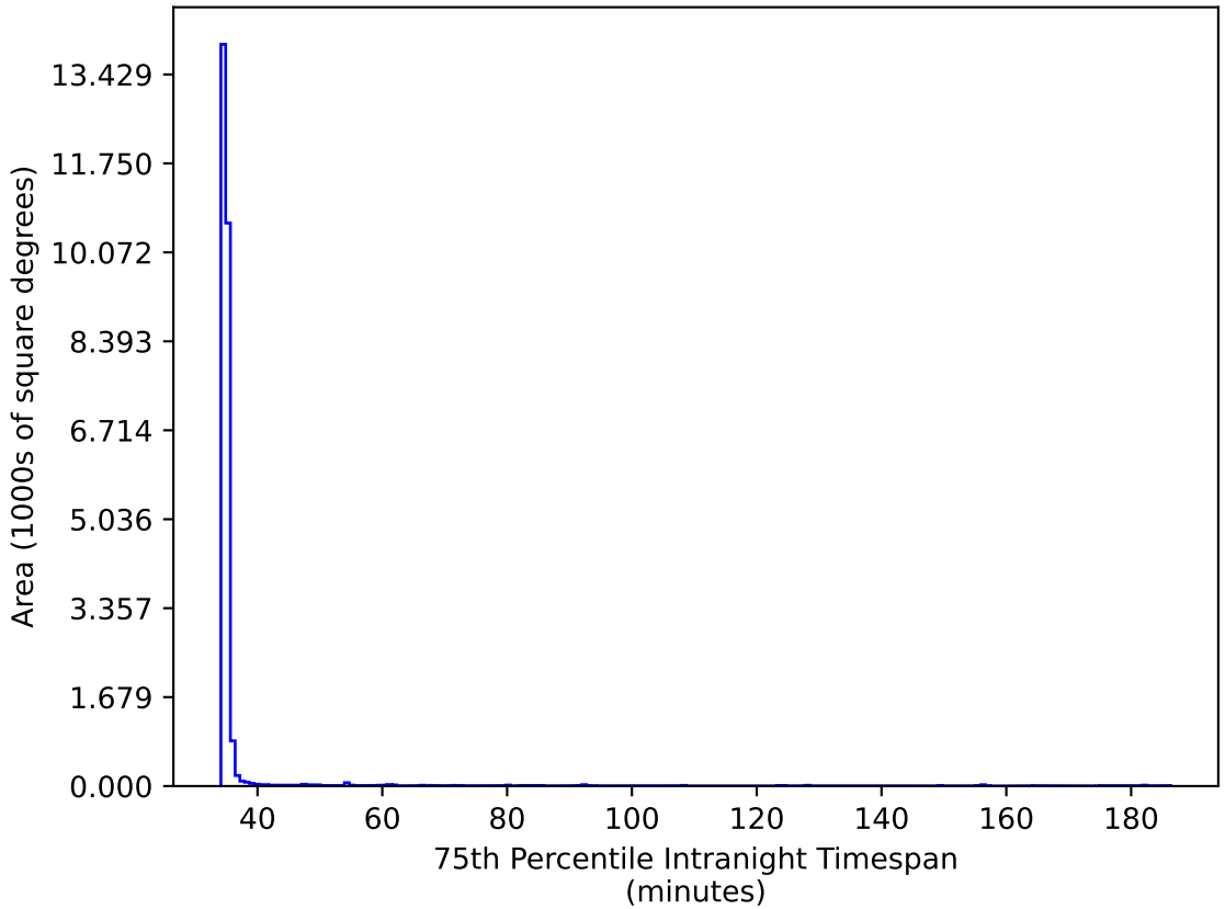
too_elab_r256_d3_griz_v3.4_10yrs All sky iz bands: 75th Percentile Intranight Timespan
