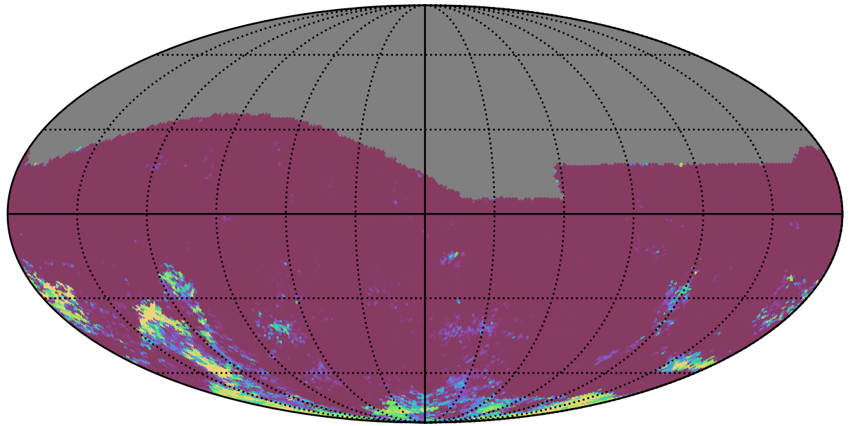
too_elab_r256_d3_griz_v3.4_10yrs All sky gr bands: 75th Percentile Intranight Timespan
