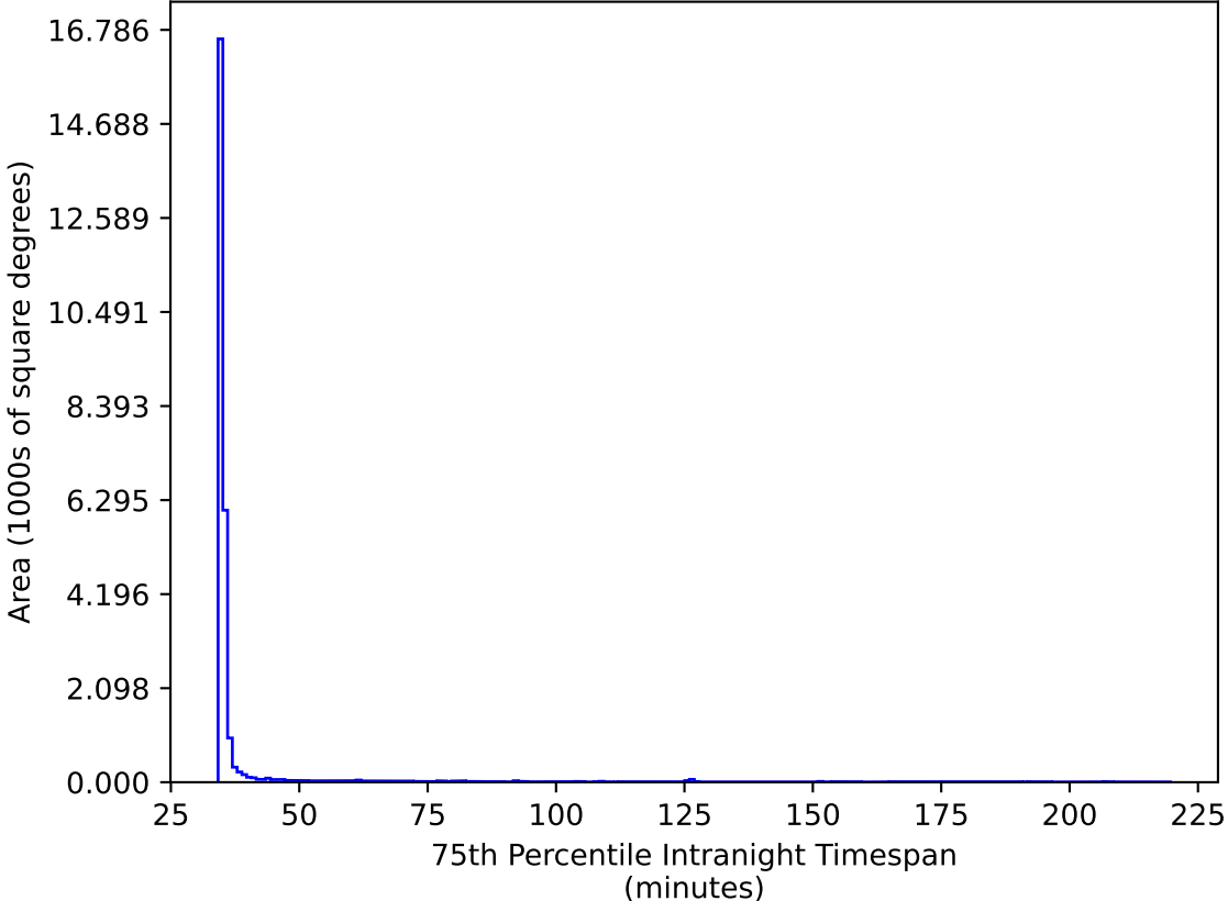
too_elab_r256_d3_griz_v3.4_10yrs All sky gr bands: 75th Percentile Intranight Timespan
