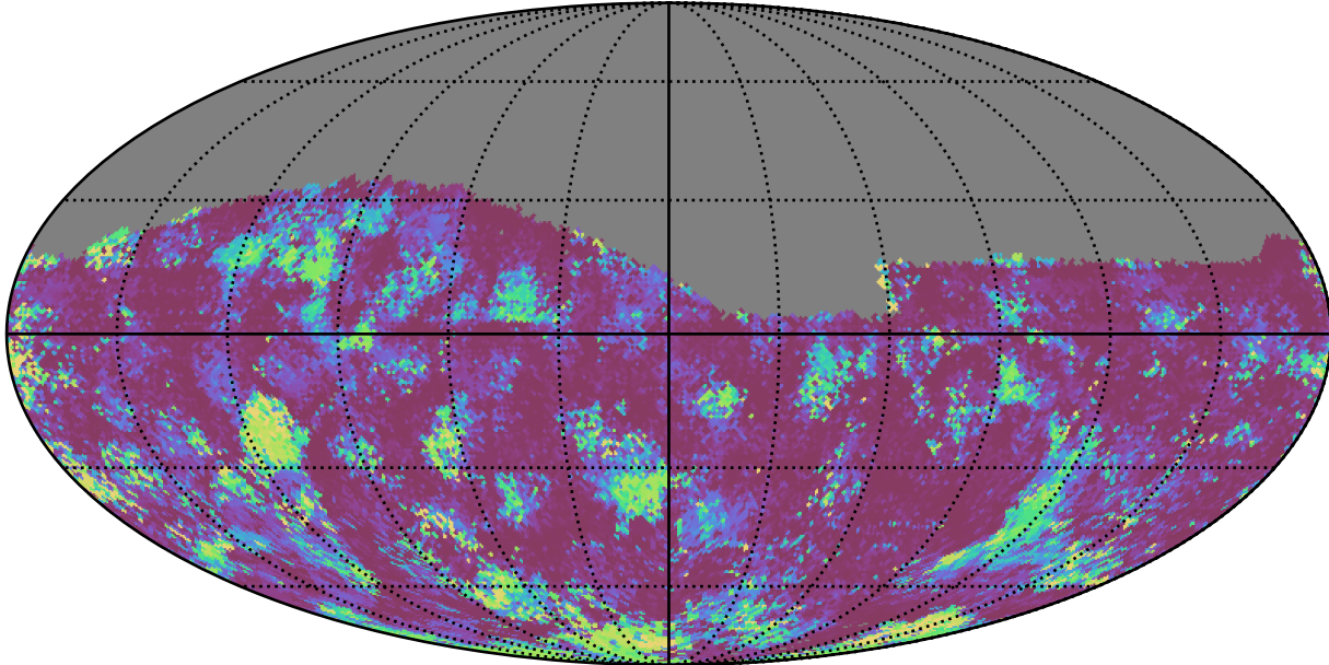
too_elab_r256_d3_griz_v3.4_10yrs All sky g band: 75th Percentile Intranight Timespan
