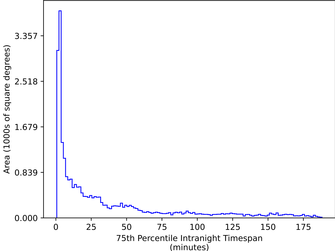
too_elab_r256_d3_griz_v3.4_10yrs All sky g band: 75th Percentile Intranight Timespan
