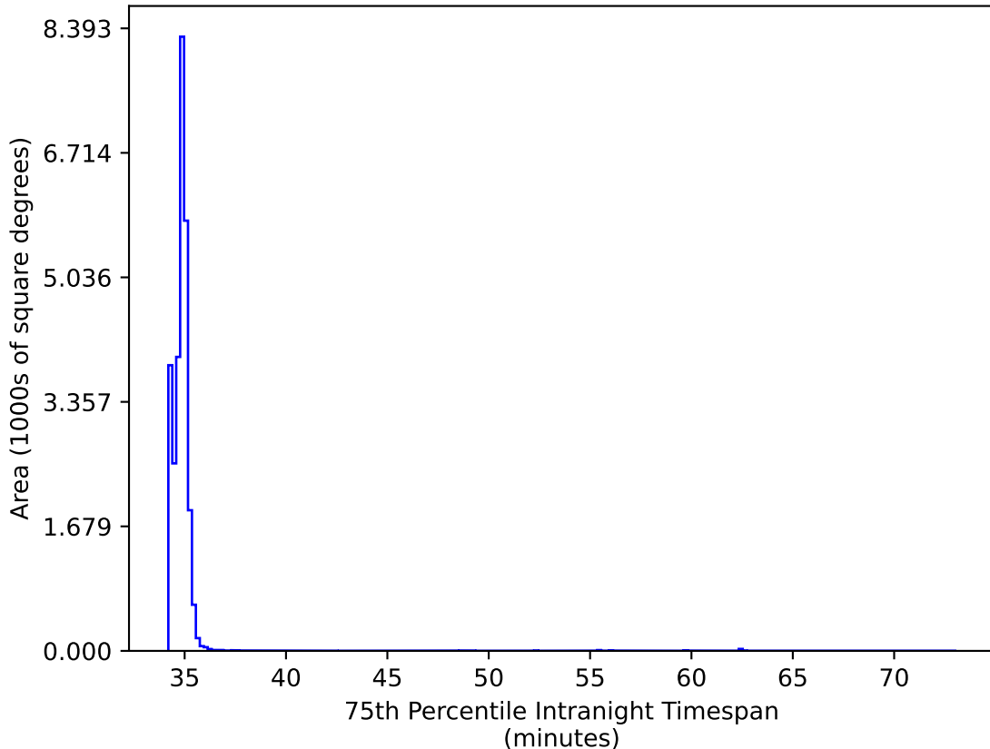
too_elab_r256_d3_griz_v3.4_10yrs All sky all bands: 75th Percentile Intranight Timespan
