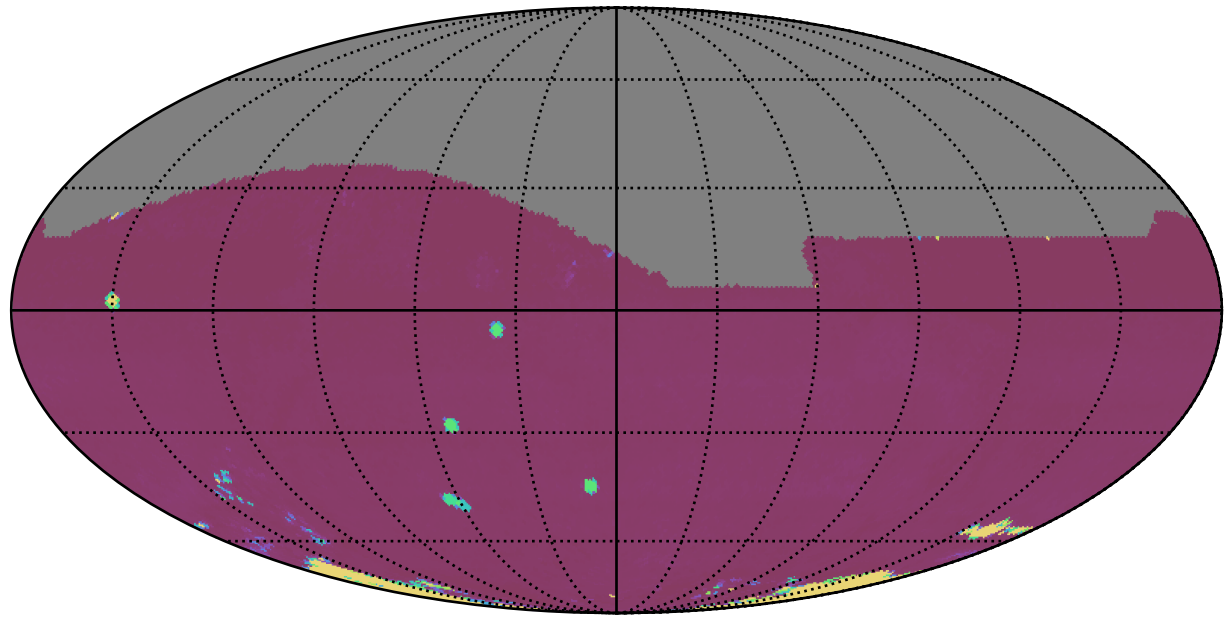
too_elab_r256_d3_griz_v3.4_10yrs All sky: 75th Percentile Intranight Timespan
