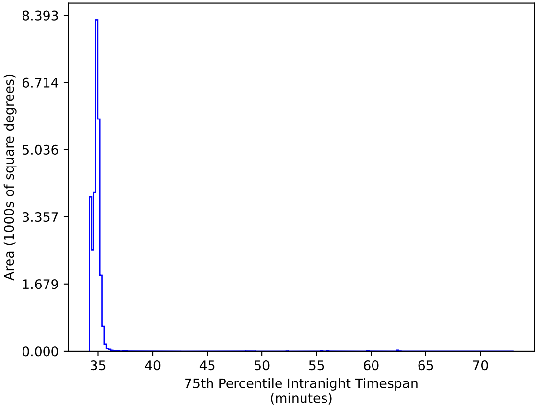
too_elab_r256_d3_griz_v3.4_10yrs All sky: 75th Percentile Intranight Timespan
