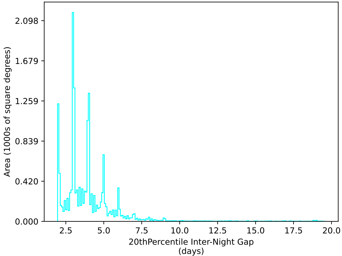
too_elab_r256_d3_griz_v3.4_10yrs WFD u band: 20thPercentile Inter-Night Gap
