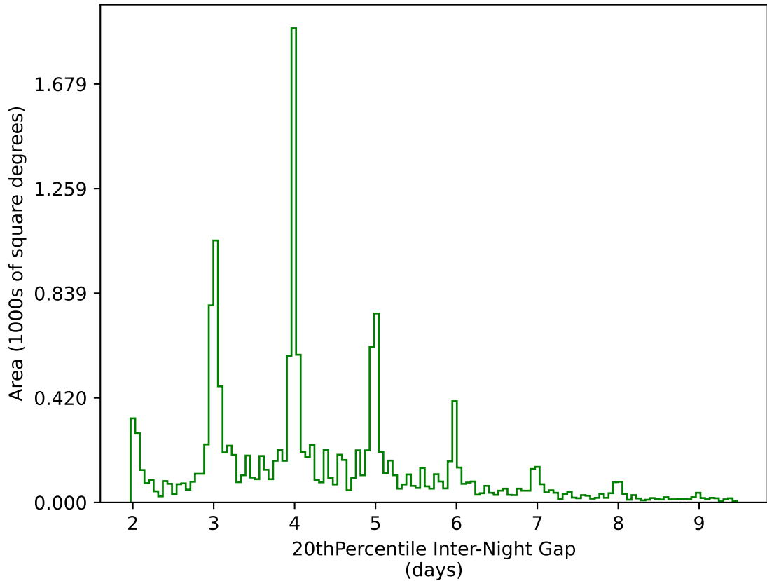
too_elab_r256_d3_griz_v3.4_10yrs WFD g band: 20thPercentile Inter-Night Gap
