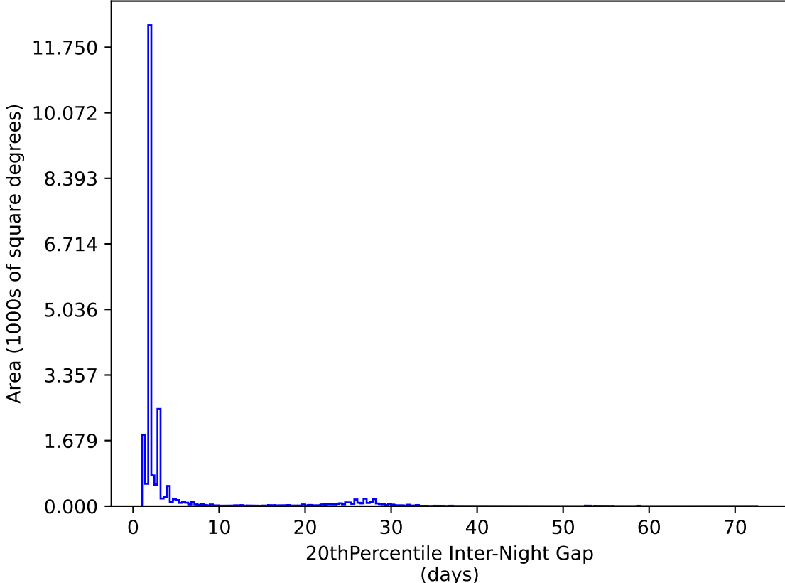
too_elab_r256_d3_griz_v3.4_10yrs All sky y band: 20thPercentile Inter-Night Gap
