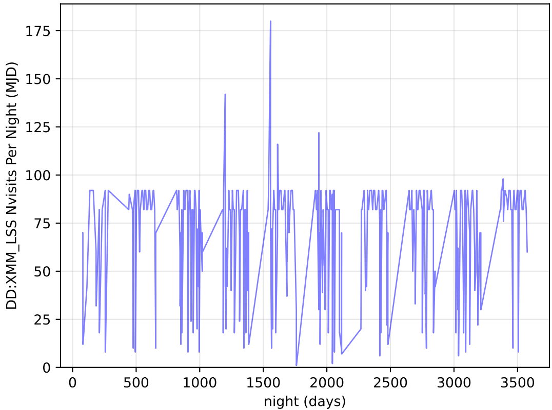
too_elab_r256_d3_griz_v3.4_10yrs all bands: DD:XMM_LSS Nvisits Per Night
