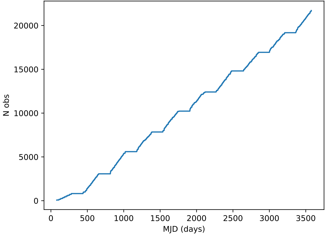
too_elab_r256_d3_griz_v3.4_10yrs all bands: DD:XMM_LSS Cumulative NVisits
