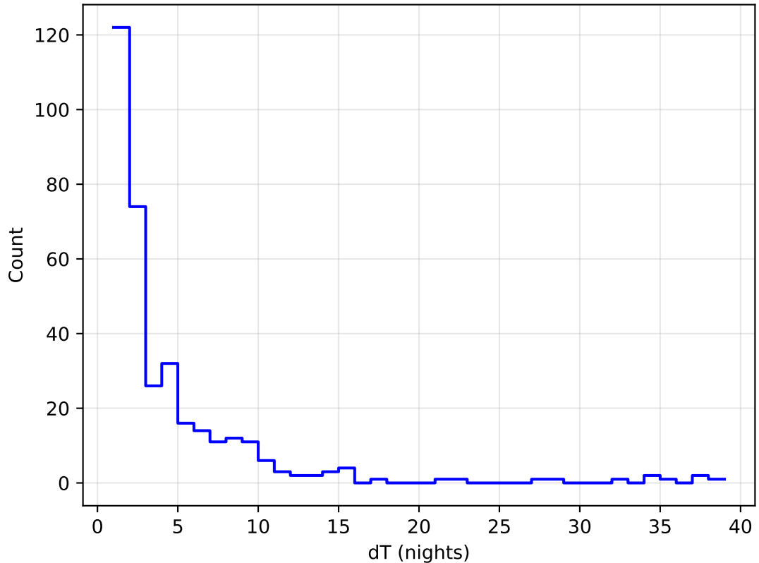
too_elab_r256_d3_griz_v3.4_10yrs all bands: DD:WFD Delta Nights Histogram
