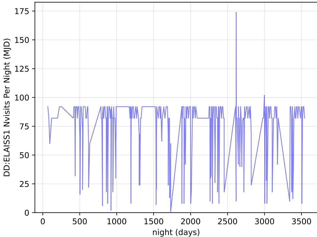
too_elab_r256_d3_griz_v3.4_10yrs all bands: DD:ELAISS1 Nvisits Per Night
