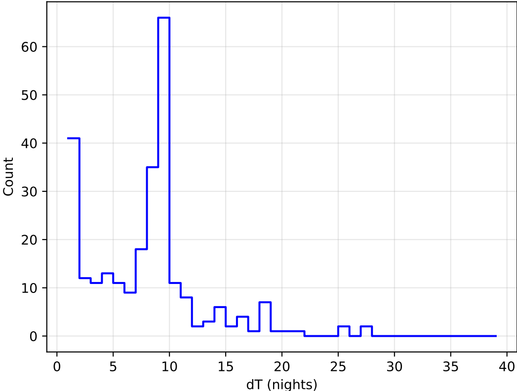
too_elab_r256_d3_griz_v3.4_10yrs all bands: DD:ELAISS1 Delta Nights Histogram
