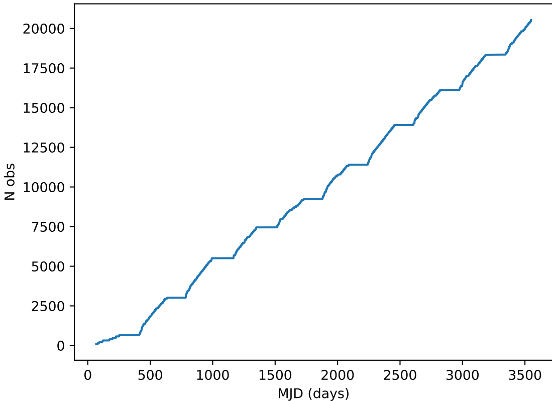
too_elab_r256_d3_griz_v3.4_10yrs all bands: DD:ELAISS1 Cumulative NVisits
