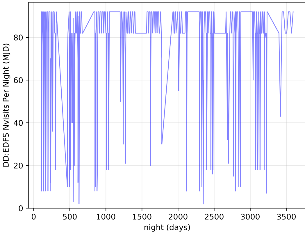
too_elab_r256_d3_griz_v3.4_10yrs all bands: DD:EDFS Nvisits Per Night
