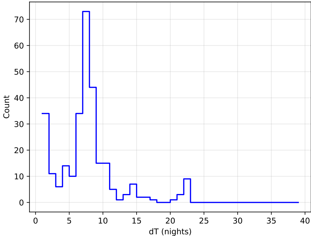
too_elab_r256_d3_griz_v3.4_10yrs all bands: DD:EDFS Delta Nights Histogram
