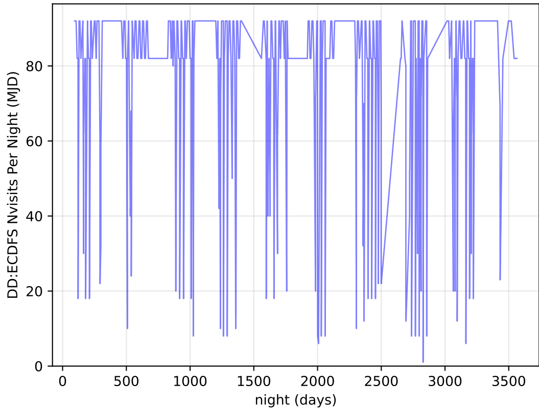
too_elab_r256_d3_griz_v3.4_10yrs all bands: DD:ECDFS Nvisits Per Night
