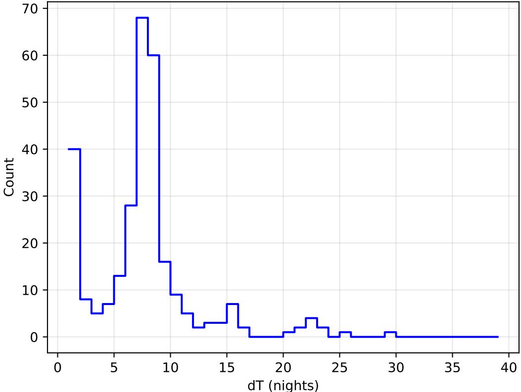
too_elab_r256_d3_griz_v3.4_10yrs all bands: DD:ECDFS Delta Nights Histogram
