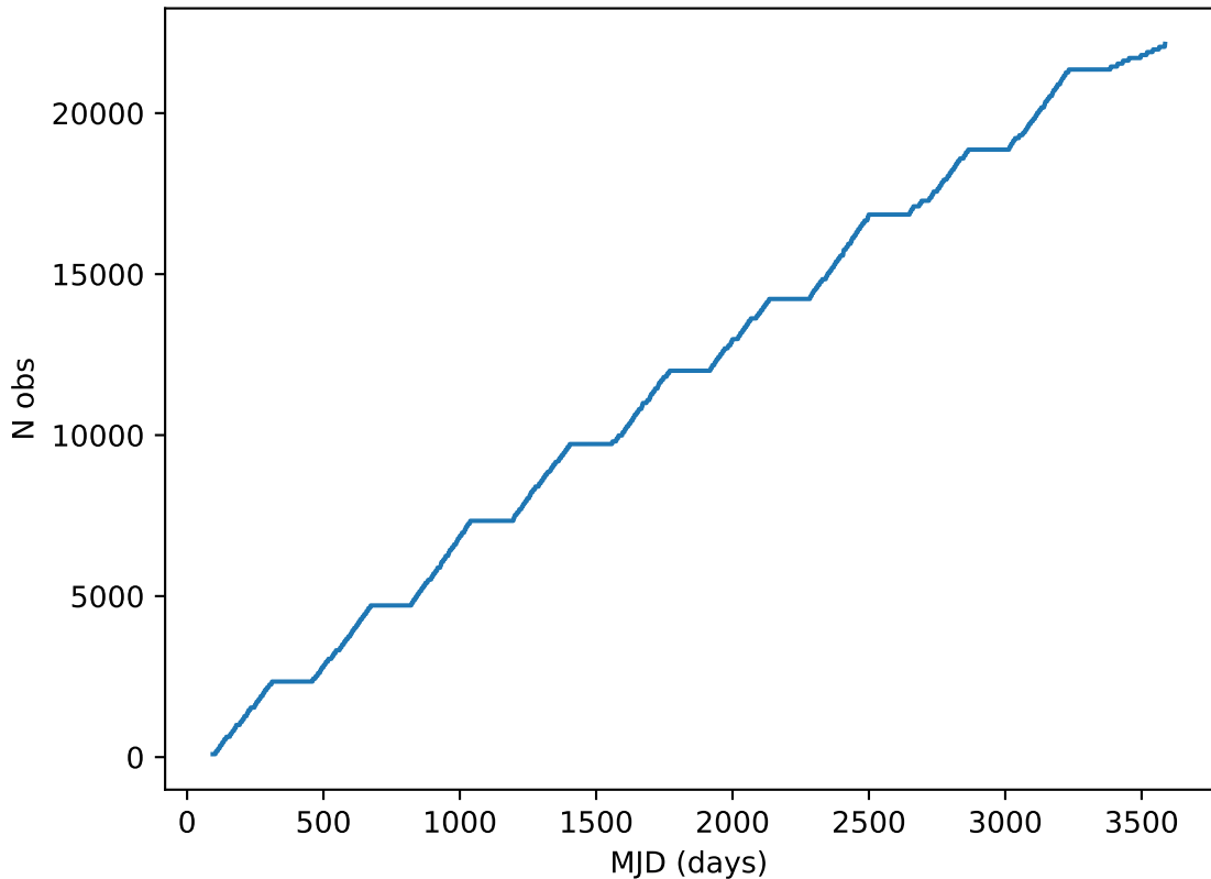
too_elab_r256_d3_griz_v3.4_10yrs all bands: DD:ECDFS Cumulative NVisits
