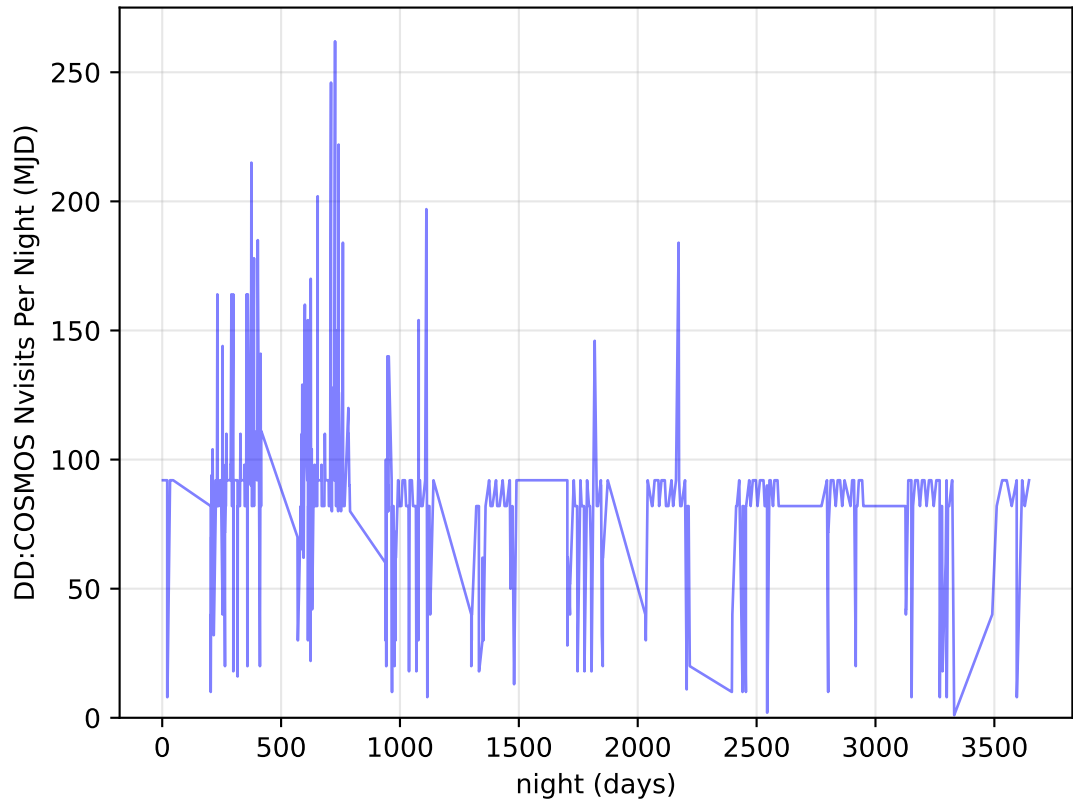
too_elab_r256_d3_griz_v3.4_10yrs all bands: DD:COSMOS Nvisits Per Night
