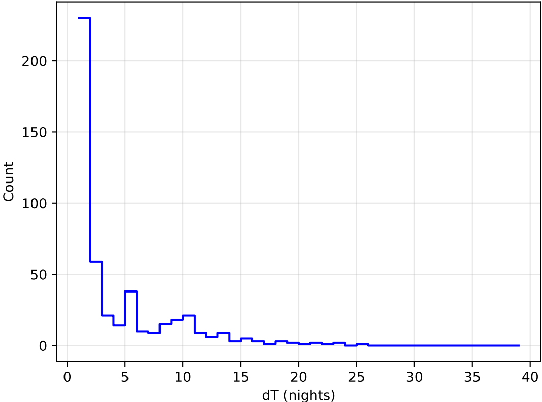
too_elab_r256_d3_griz_v3.4_10yrs all bands: DD: COSMOS Delta Nights Histogram
