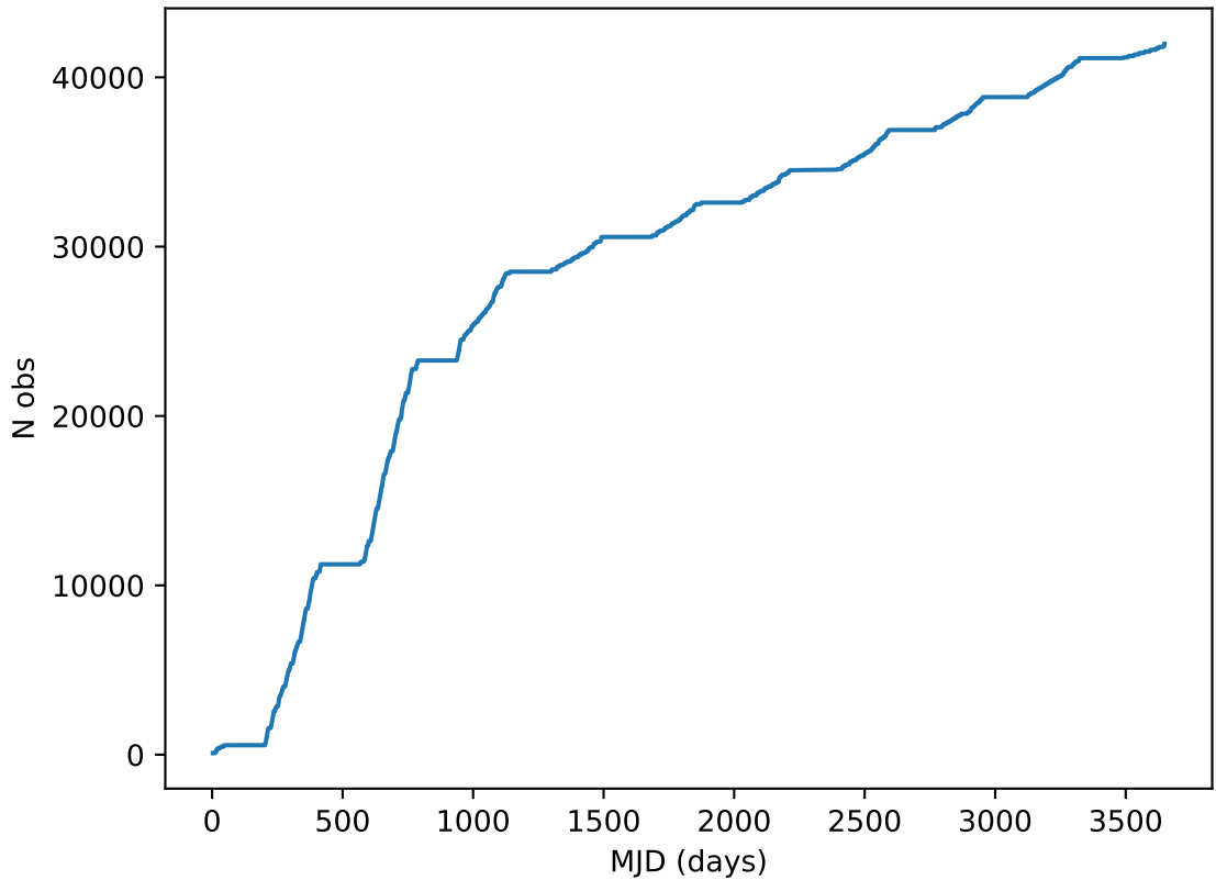
too_elab_r256_d3_griz_v3.4_10yrs all bands: DD: COSMOS Cumulative NVisits
