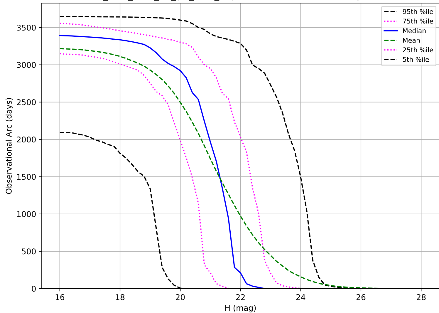
too_elab_r256_d3_giz_v3.4_10yrs: Observational Arc Length PHA
