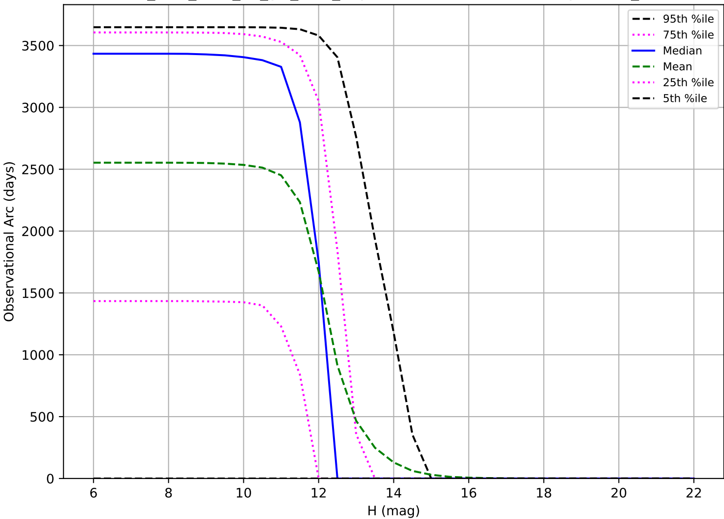
too_elab_r256_d3_giz_v3.4_10yrs: Observational Arc Length OCC_r20
