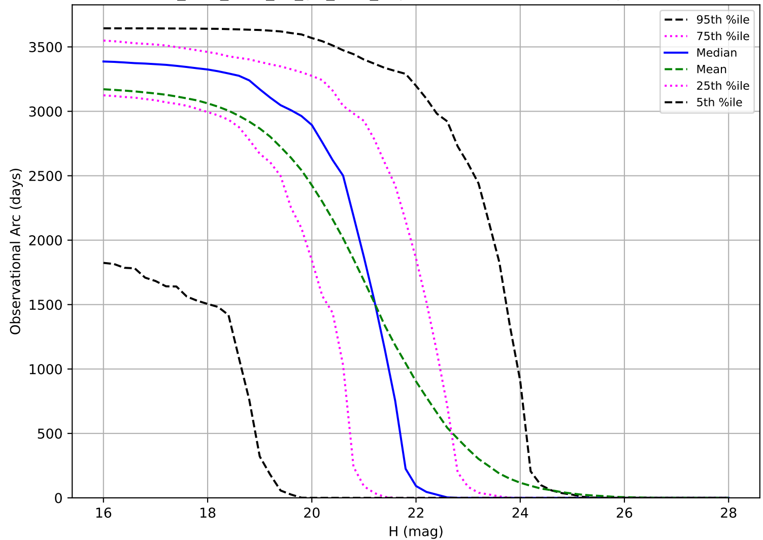
too_elab_r256_d3_giz_v3.4_10yrs: Observational Arc Length NEO
