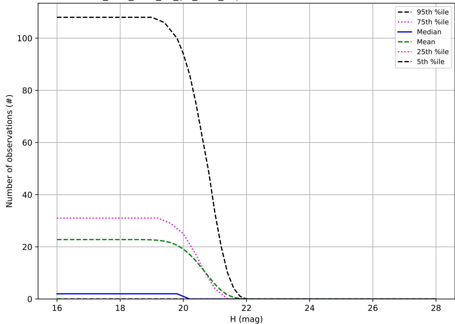
too_elab_r256_d3_giz_v3.4_10yrs: Number of observations Vatira
