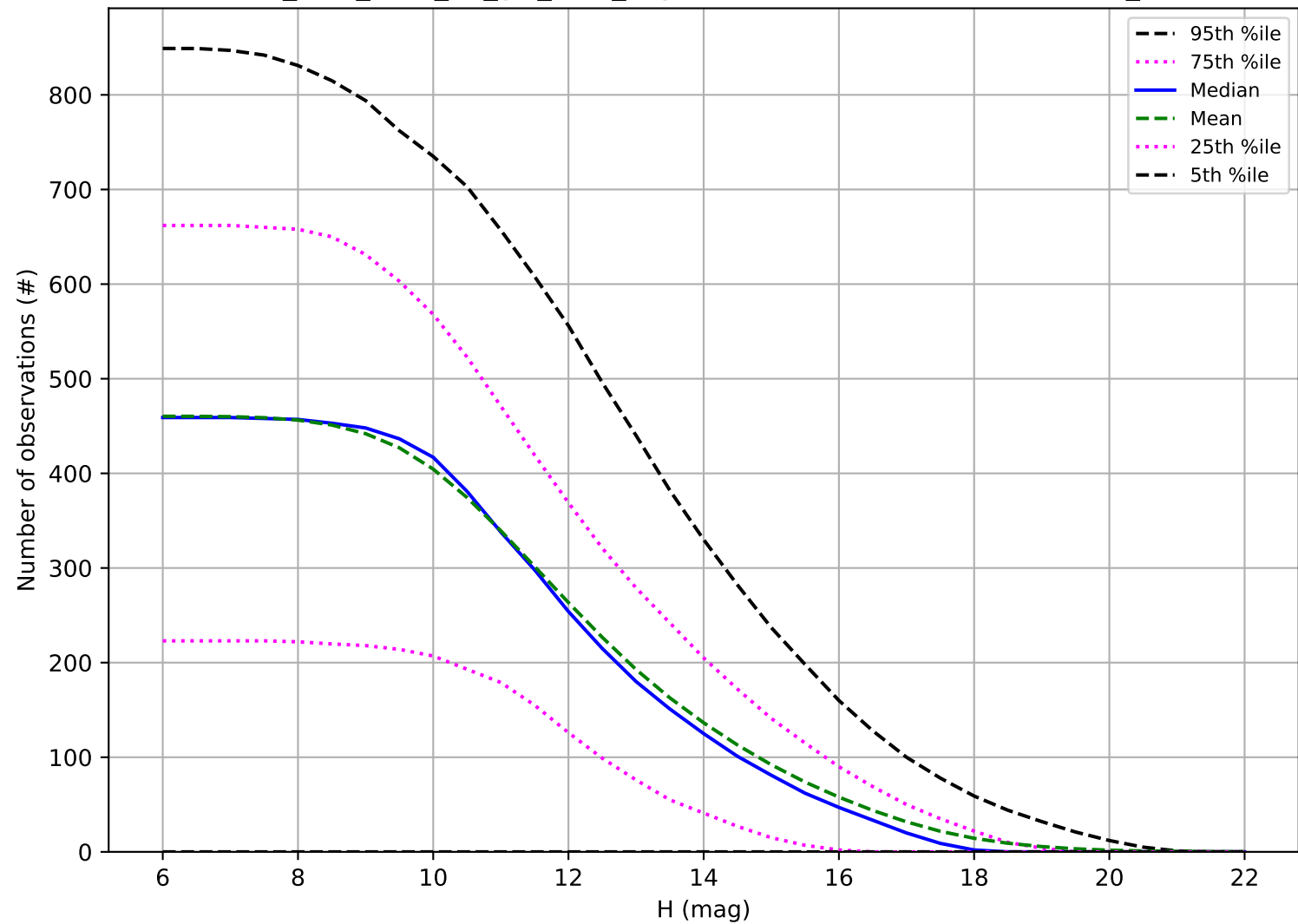
too_elab_r256_d3_giz_v3.4_10yrs: Number of observations OCC_r5
