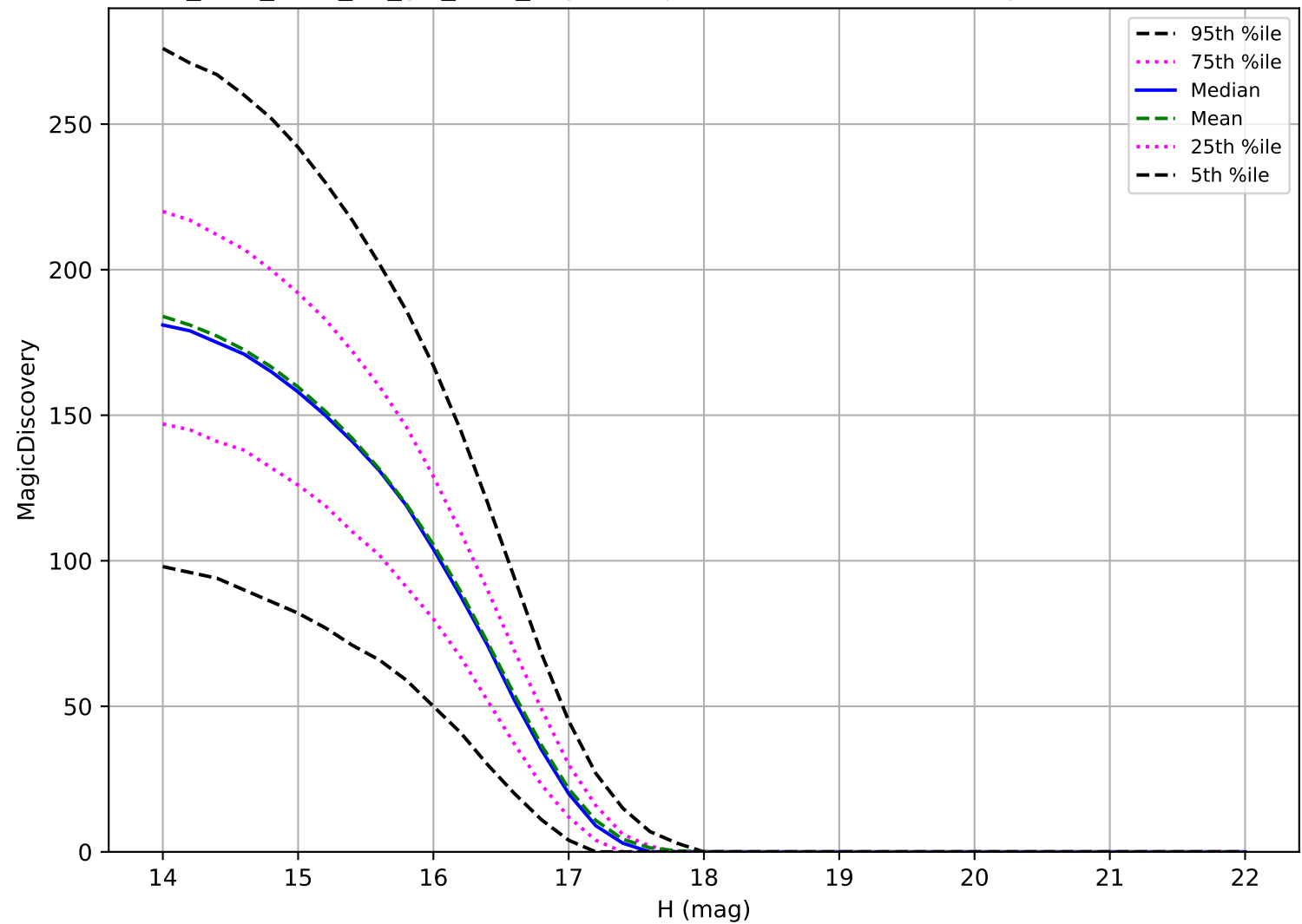
too_elab_r256_d3_giz_v3.4_10yrs: Trojan 6 detections in 60 nights detection loss
