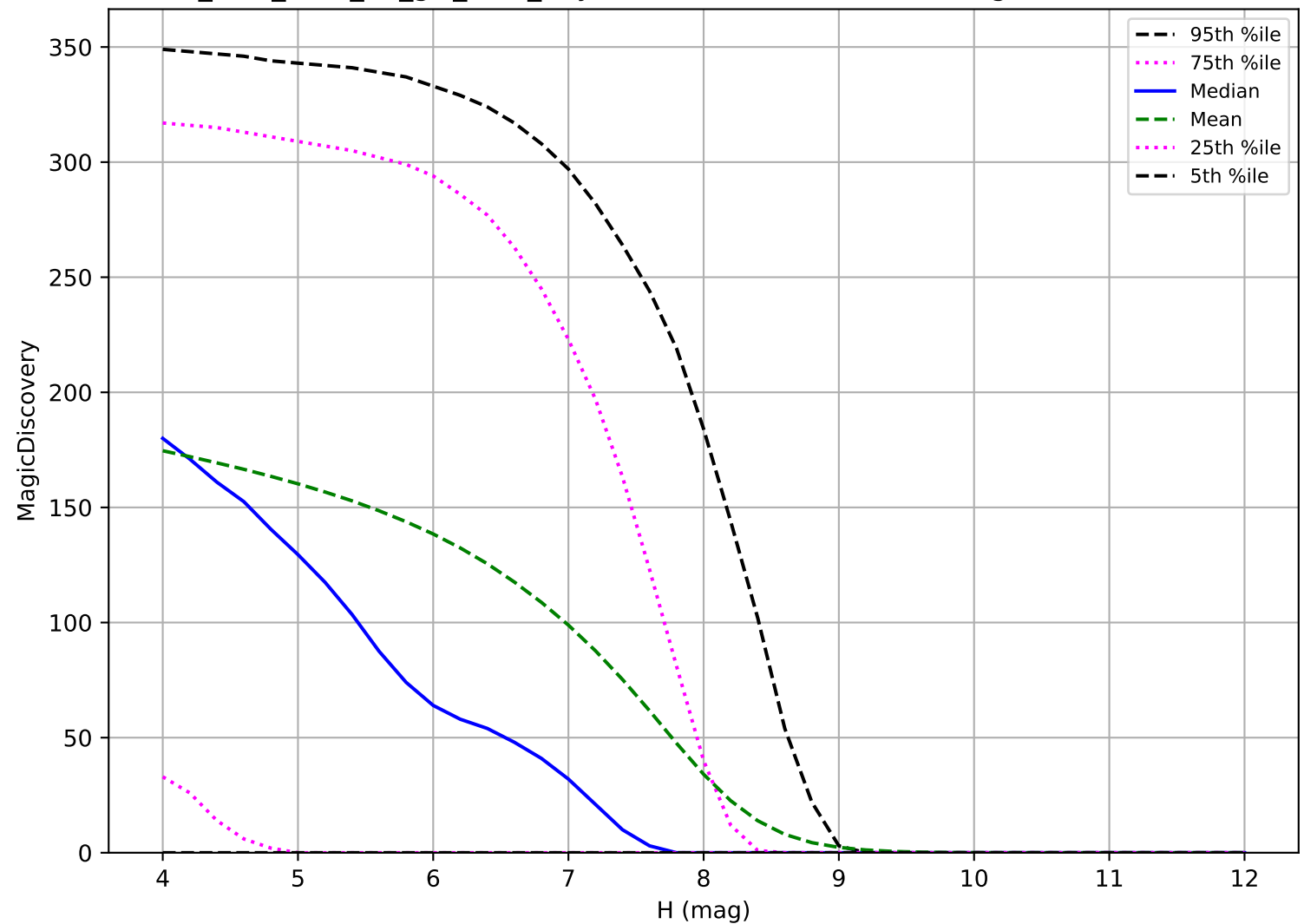
too_elab_r256_d3_giz_v3.4_10yrs: TNO 6 detections in 60 nights detection loss
