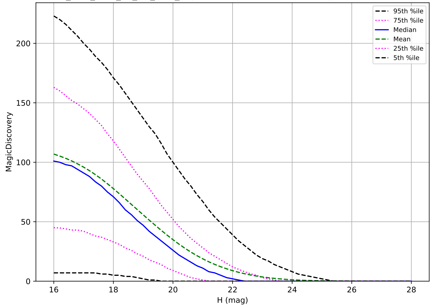
too_elab_r256_d3_giz_v3.4_10yrs: PHA 6 detections in 60 nights detection loss
