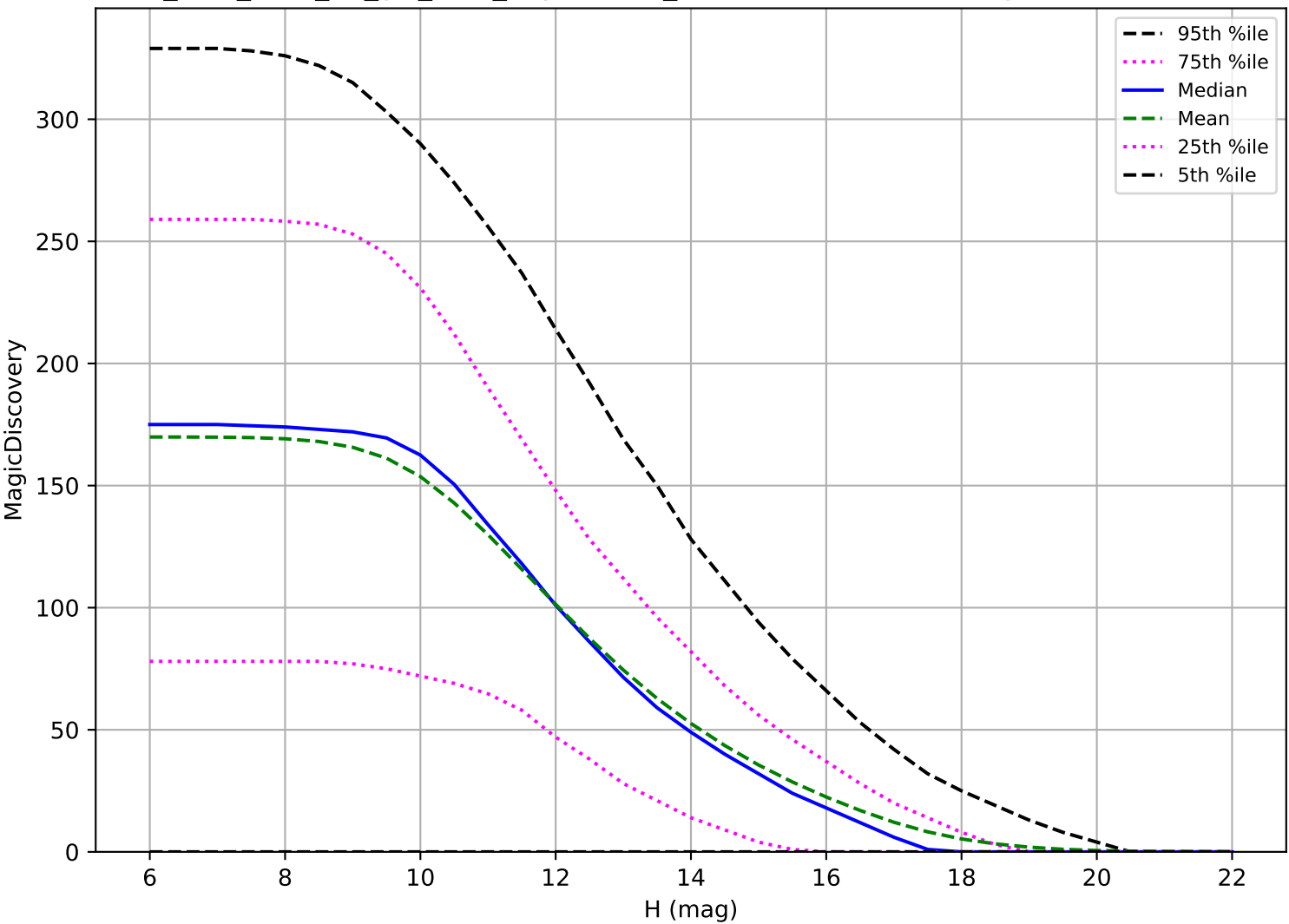
too_elab_r256_d3_giz_v3.4_10yrs: OCC_r5 6 detections in 60 nights detection loss
