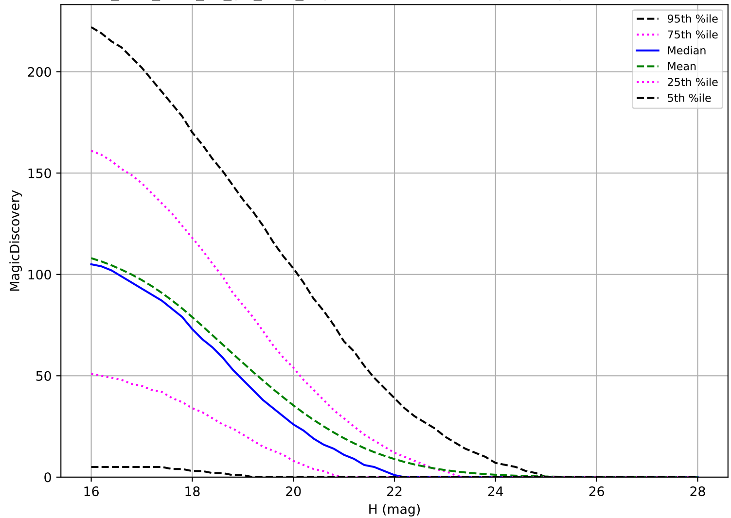
too_elab_r256_d3_giz_v3.4_10yrs: NEO 6 detections in 60 nights detection loss
