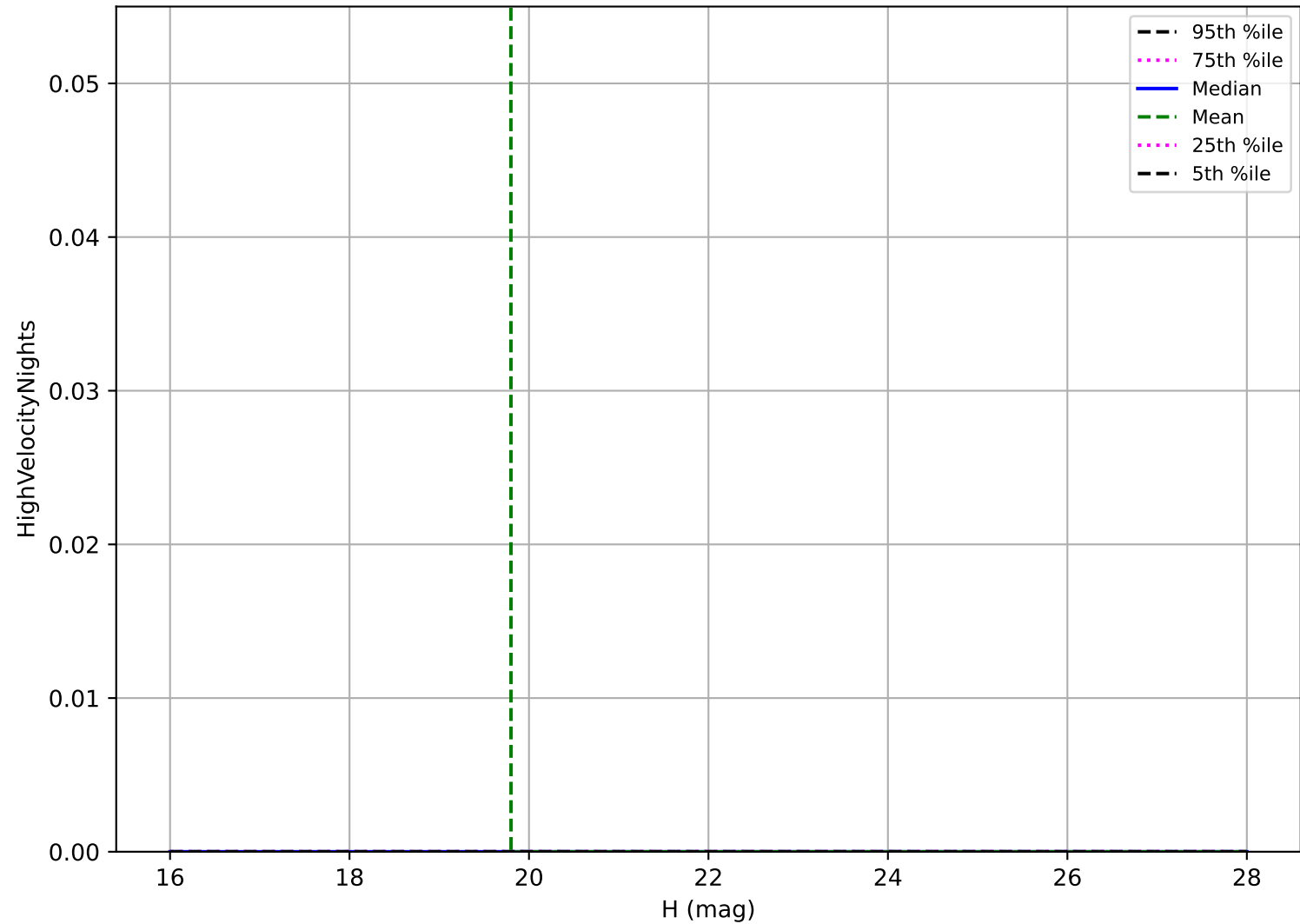
too_elab_r256_d3_giz_v3.4_10yrs: Vatira High velocity pair detection loss
